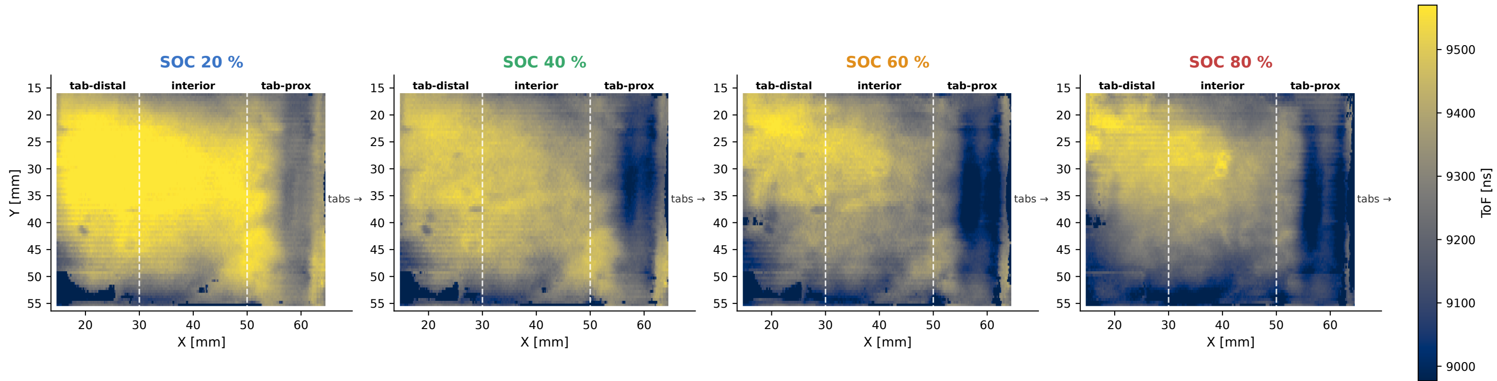
Figure C End-of-rest ToF maps (ROI only) at each SOC plateau shared scale 8977-9570 ns; dashed lines at X = 30, 50 mm divide sub-regions
