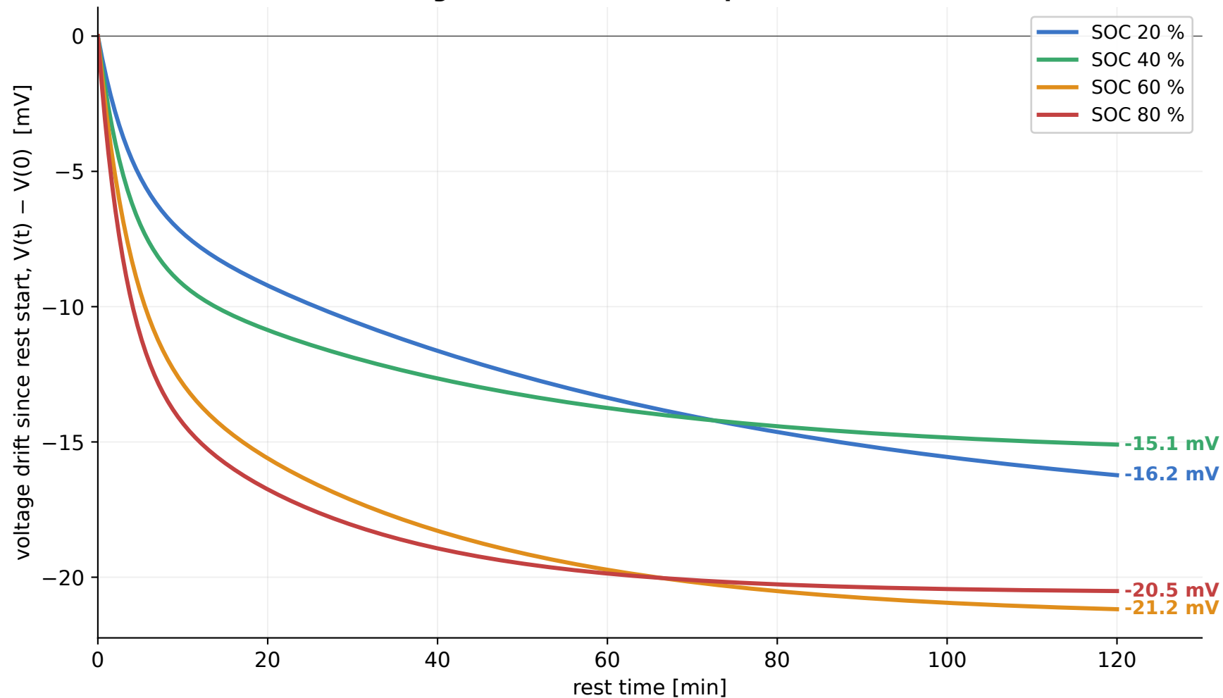
OCV drift during 2 h rest at each SOC plateau (35 °C, smoothed)
