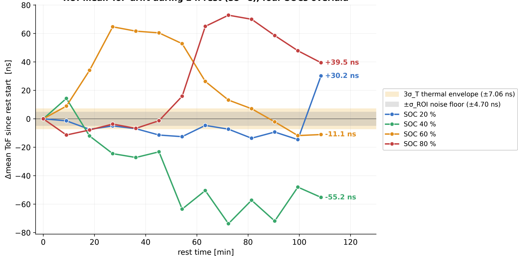
ROI-mean ToF drift during 2 h rest (35 °C), four SOC's overlaid
