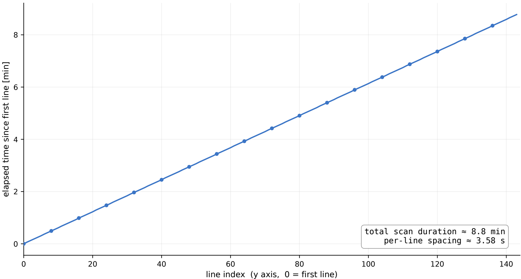
Figure F Per-line acquisition time within one scan (supports: acquisition-time gradient is in y, not x)
