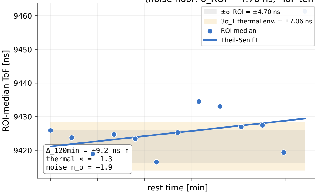
Figure A Rest evolution of cell-ROI for , per SOC plateau (noise floor: \sigma_{ROI} = 4.70 ns; ToF temperature coefficient: \alpha_T = +73.5 ns/°C)
