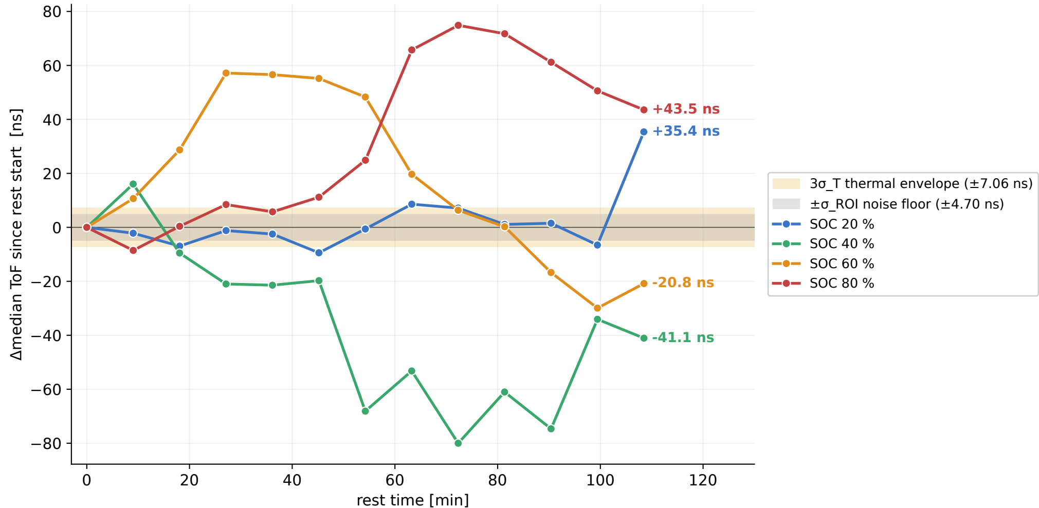
ROI-median ToF drift during 2 h rest (35 °C), four SOC levels overlaid
