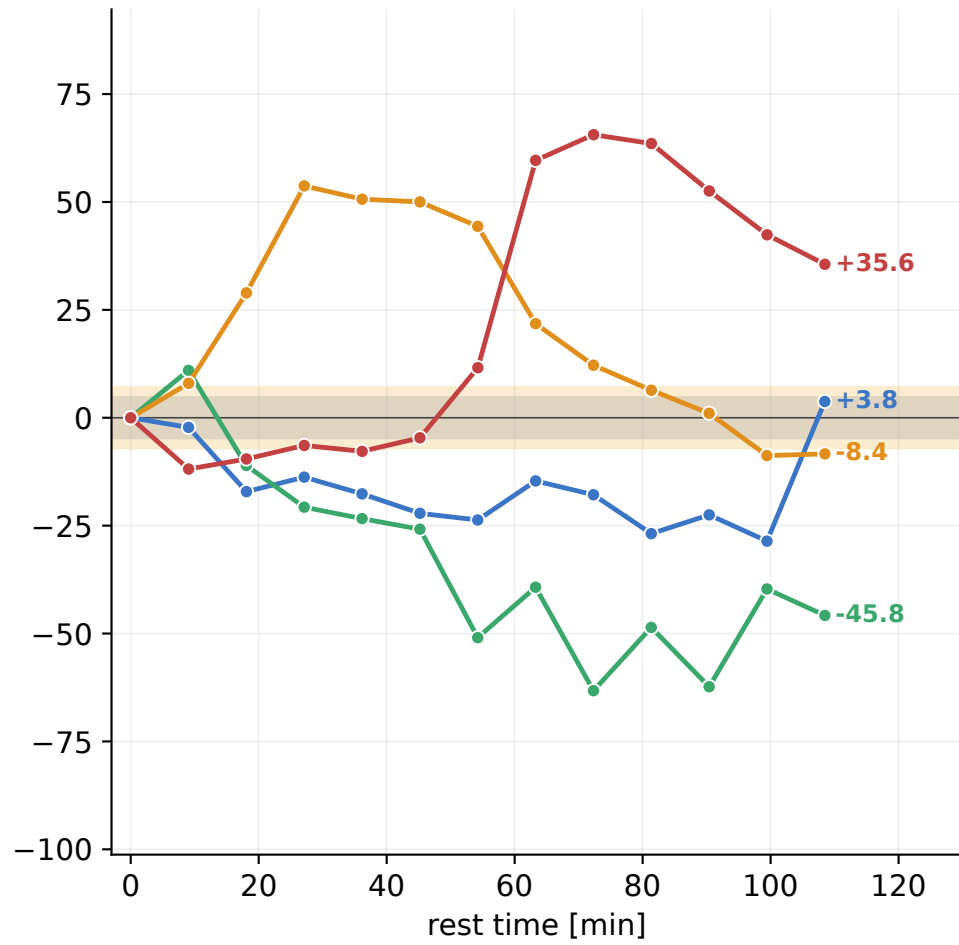
tab-distal X = 14.6-30.0 mm
