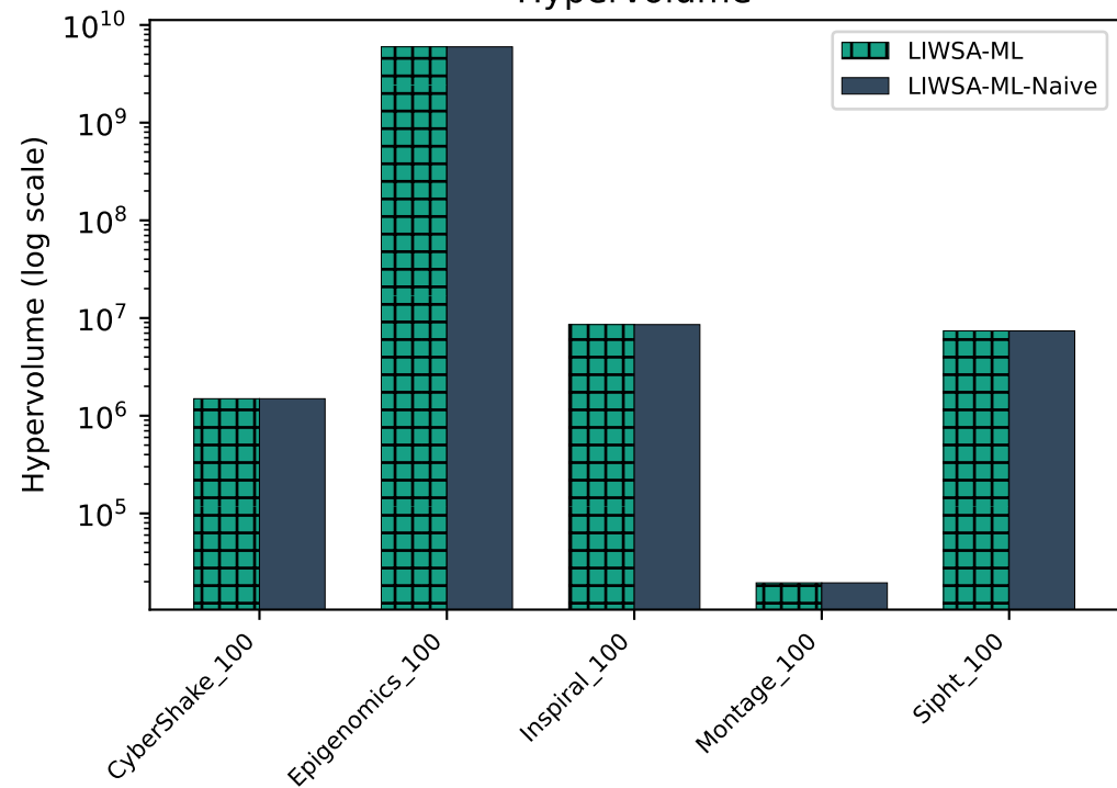
Hypervolume
