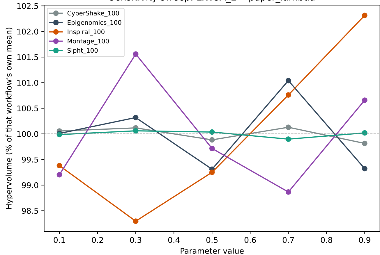
Sensitivity sweep: LIWSA_L -- paper_lambda
