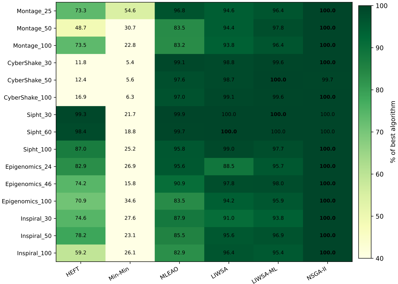
Hypervolume, % of the best algorithm -- small and medium instances (24-100 tasks)
