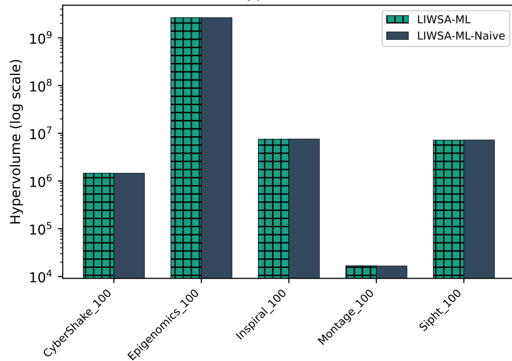
Hypervolume
