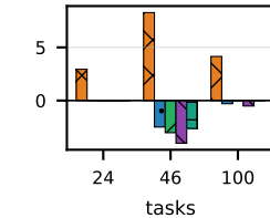
Epigenomics
