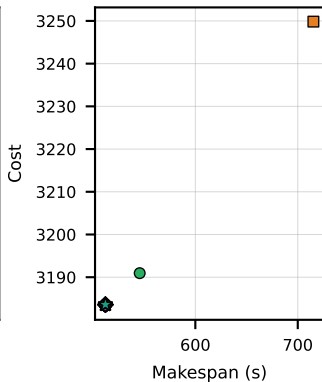
CyberShake_100
