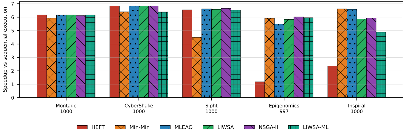
Scheduling speedup on large workflow instances
