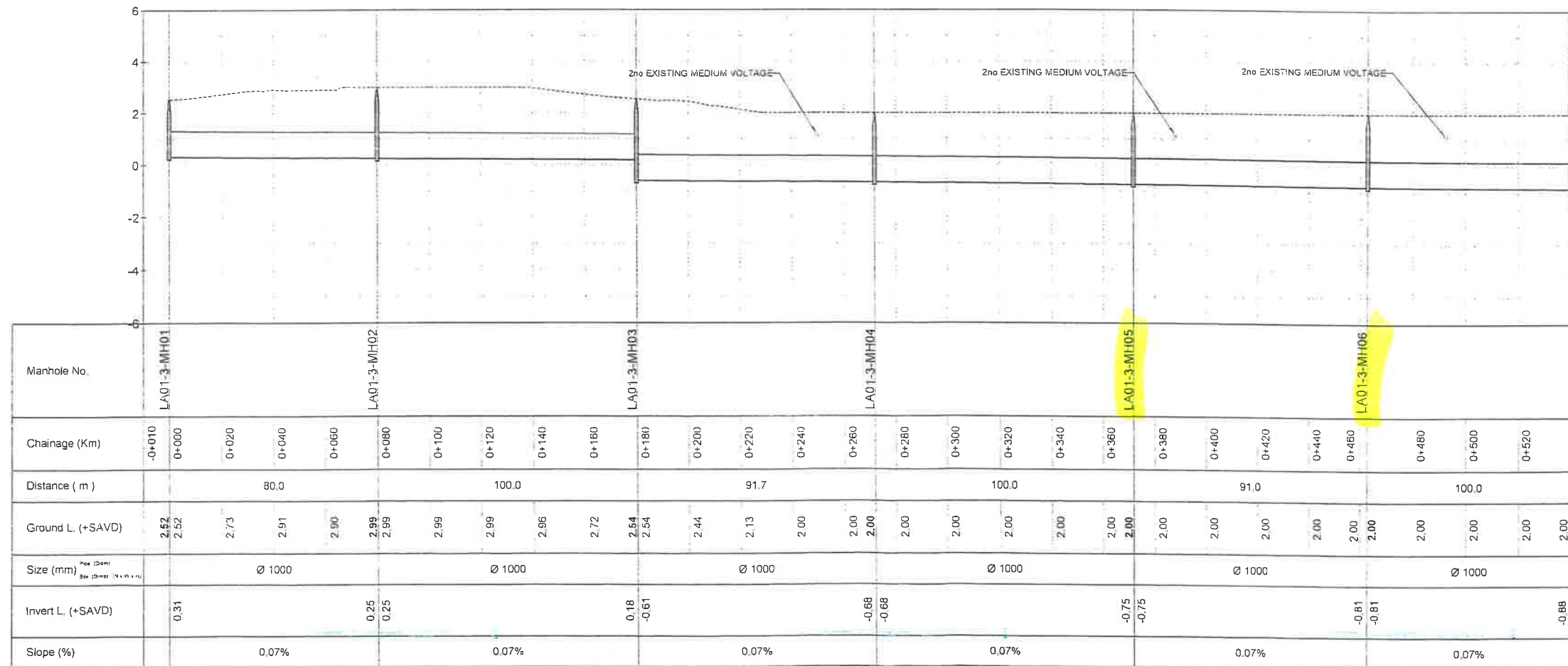
PROFILE L01-3
