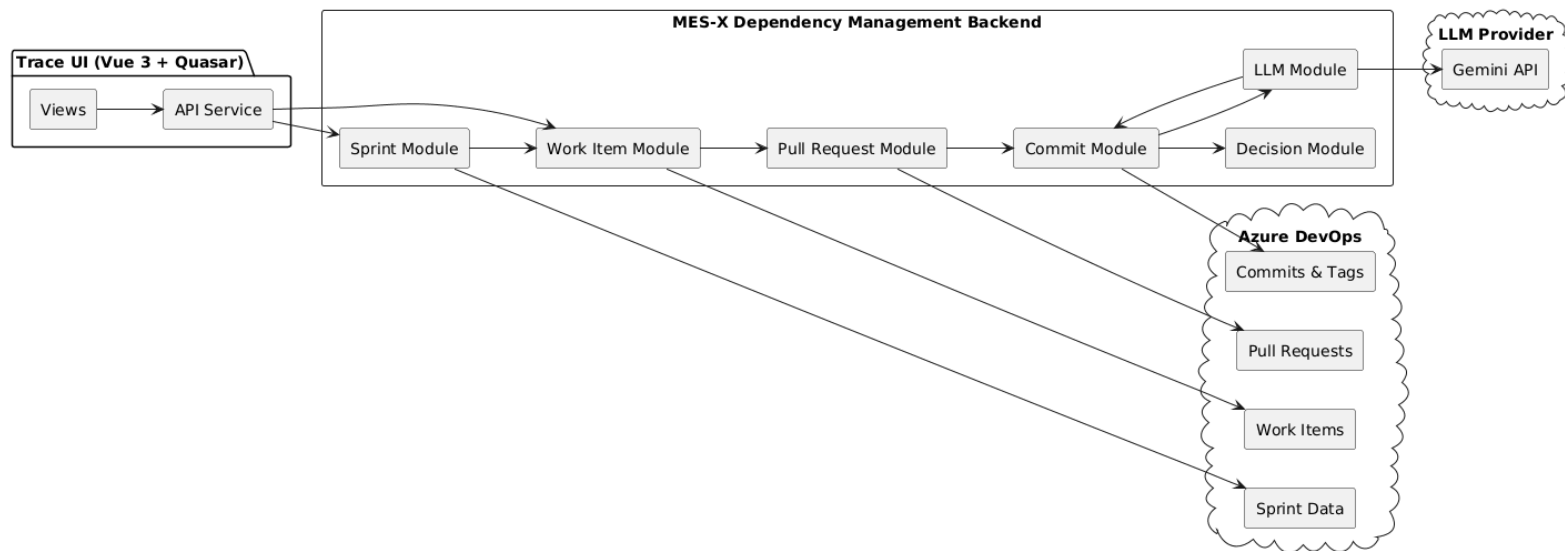
Figure 4.3: Global connection graph of the Trace UI and backend modules
