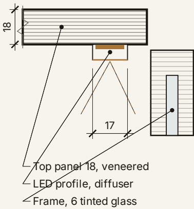
02 HEAD DETAIL 1 : 2
