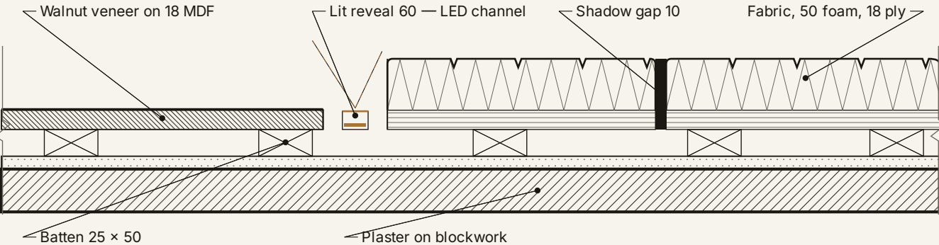
02 CD-02 WALNUT / LIT REVEAL / UPHOLSTERY — PLAN SECTION NTS · CONCEPT DETAIL · TYPICAL SIZES · READS FIG. 05
