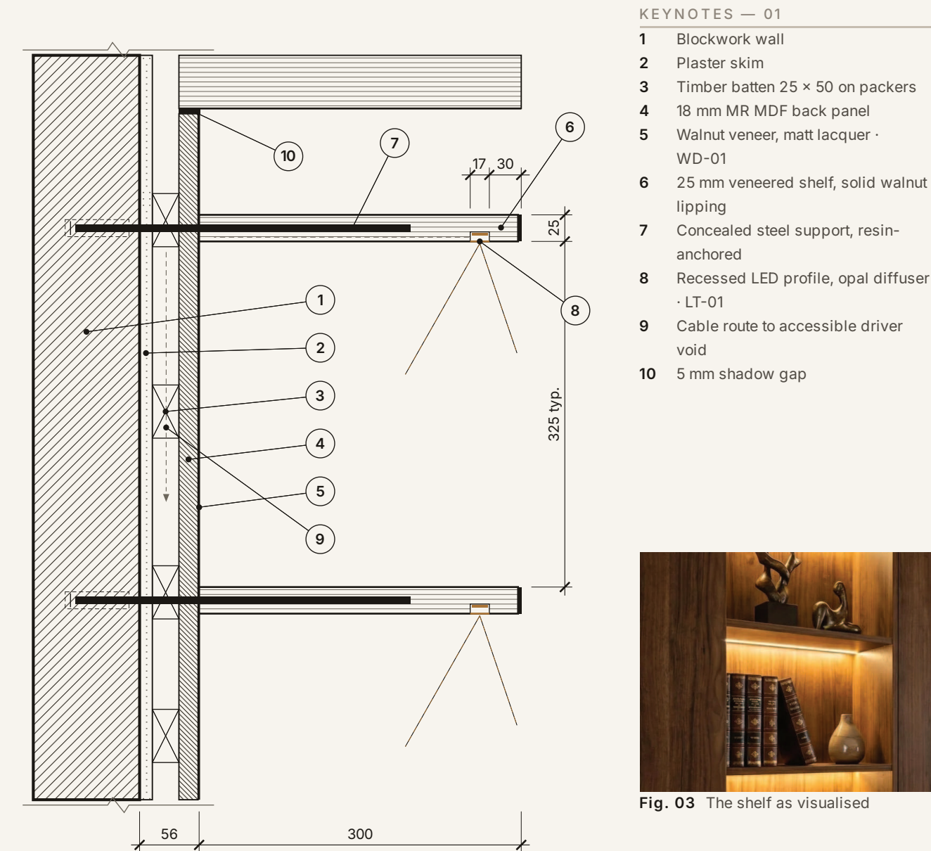
01 CD-01 LIT SHELF — SECTION NTS · CONCEPT DETAIL · TYPICAL SIZES
