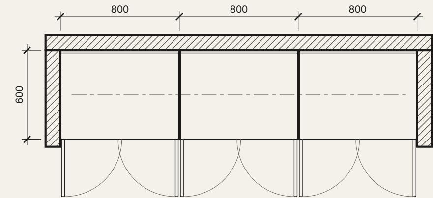
03 PLAN RE-02 1 : 25
