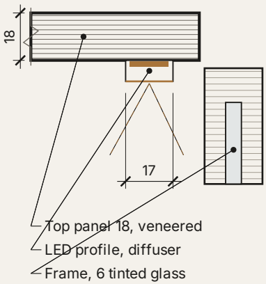
02 HEAD DETAIL RE-02 1 : 2
