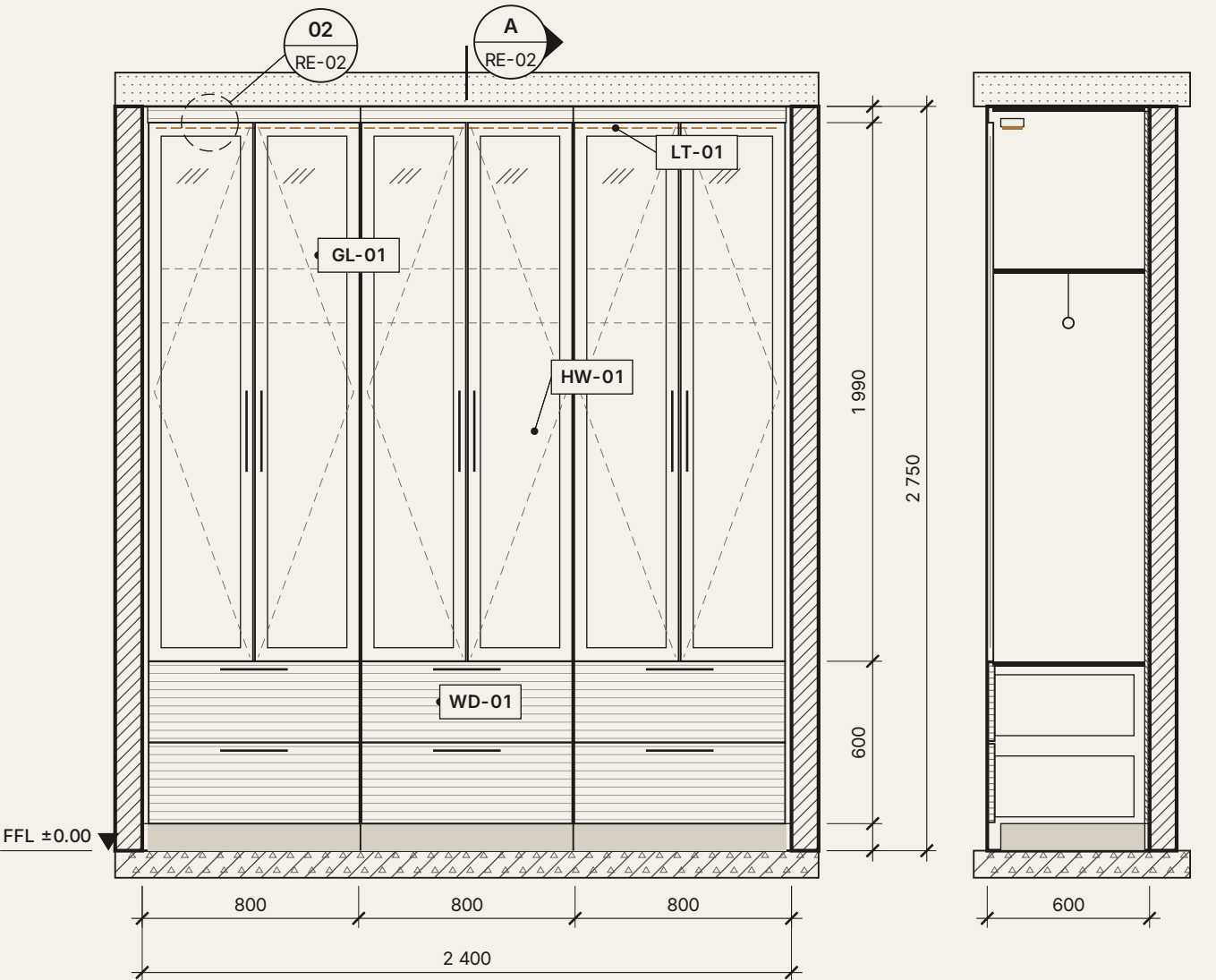
01 FRONT ELEVATION RE-02 1 : 25 · TYPICAL
