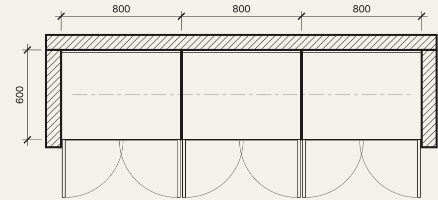
03 PLAN RE-02 1: 25
