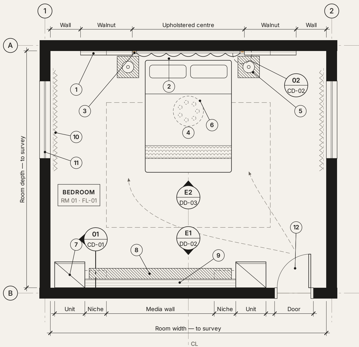
01 DD-01 LAYOUT READING — BEDROOM NTS · CONCEPTUAL SPACE STUDY · READS FIG. 01 + 02
