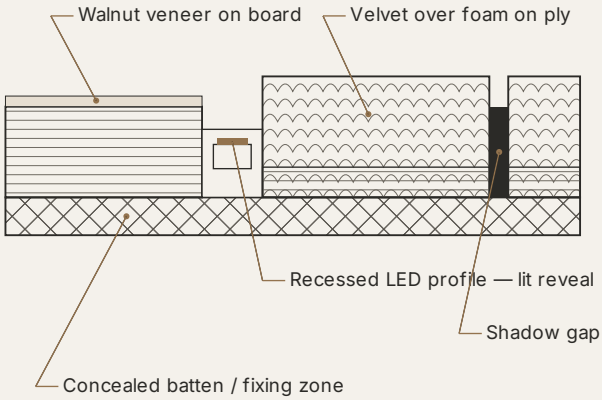
THE WALNUT SUITE · READS FIG. 05 Walnut/light/velvet junction — plan CONCEPT DETAIL CD-01 · NTS
