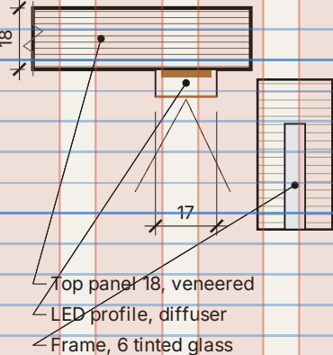
02 HEAD DETAIL
