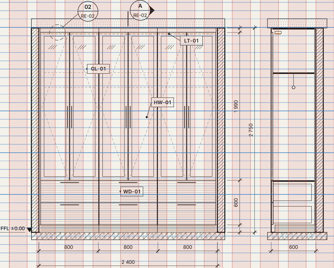
01 FRONT ELEVATION
