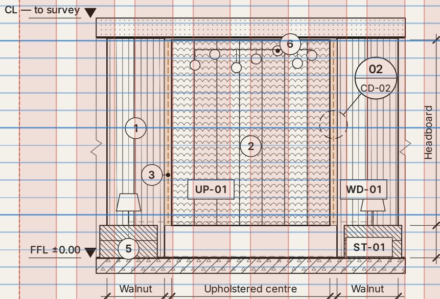
E2 HEADBOARD WALL — ELEVATION DD-03
