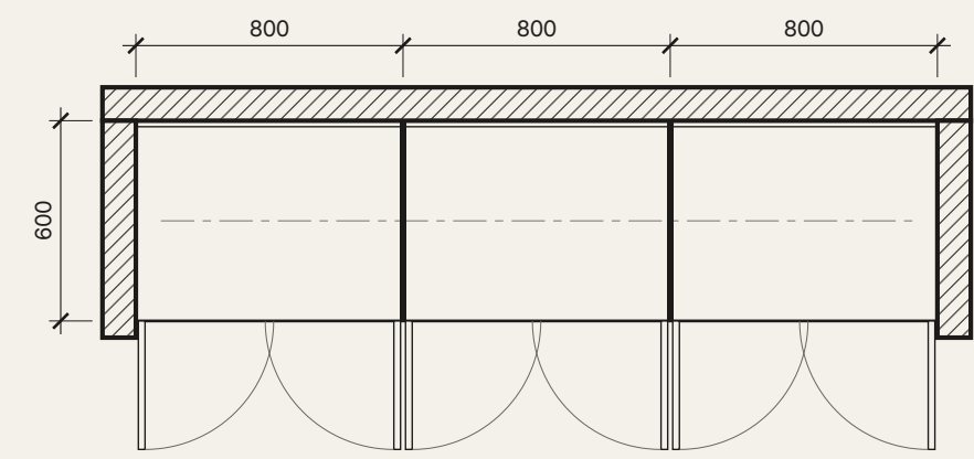
03 PLAN 1: 25
