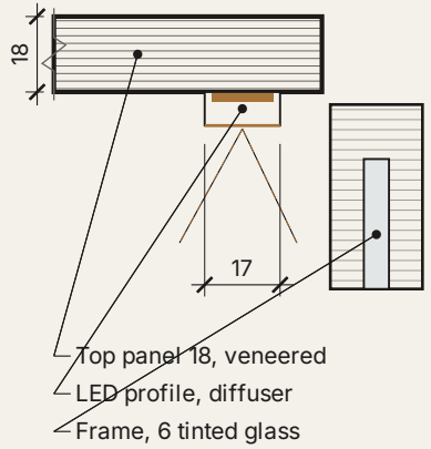
02 HEAD DETAIL 1: 2
