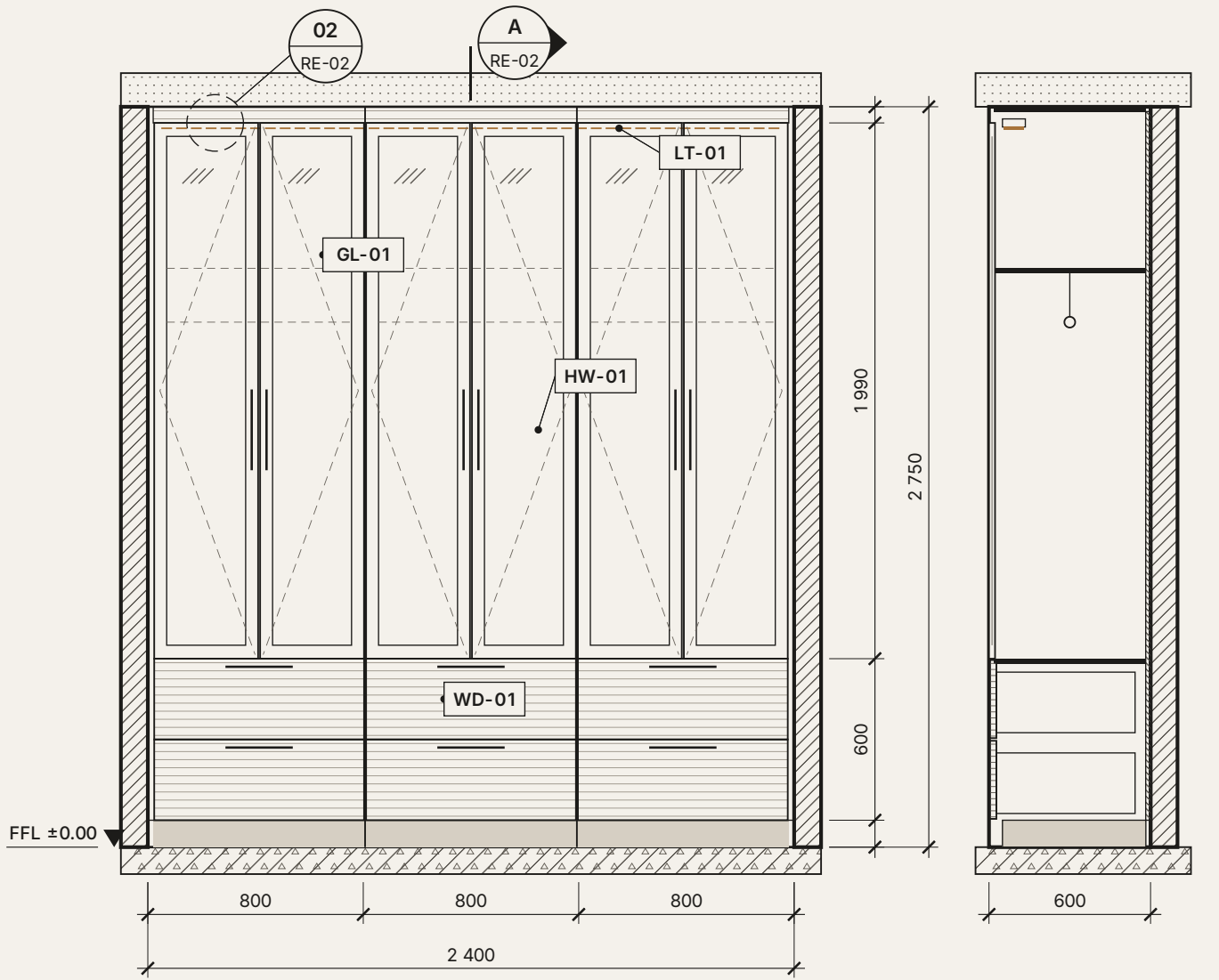
01 FRONT ELEVATION 1: 25 · TYPICAL
