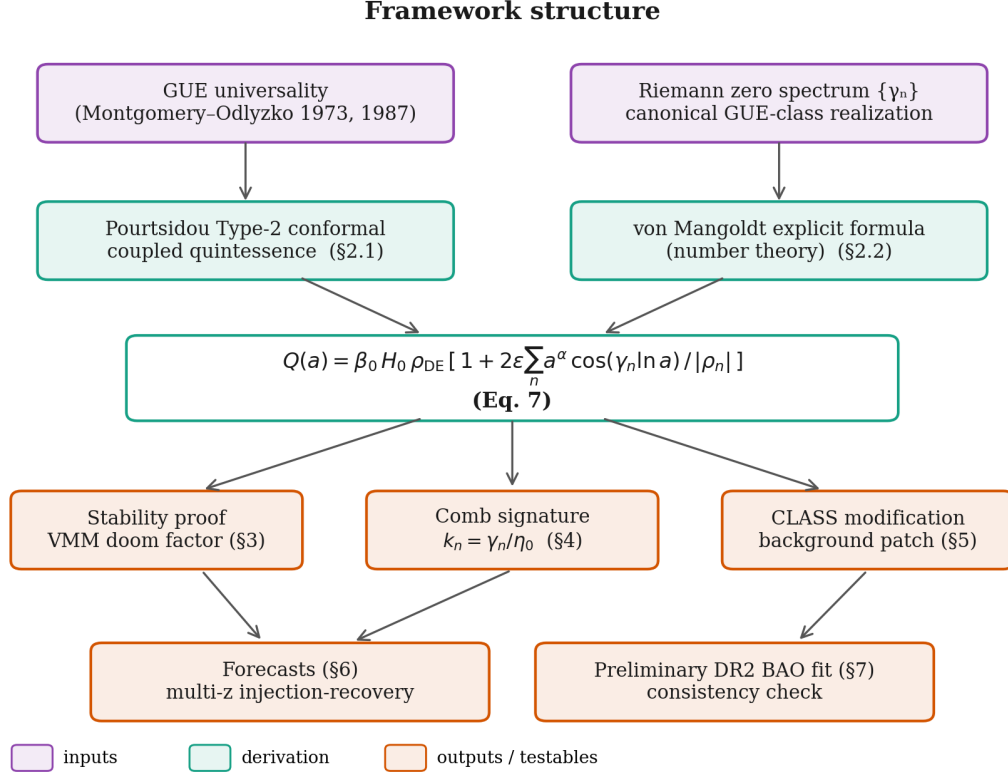
Figure 1: Logical structure of the framework: GUE-motivated ansatz + Type-2 coupled-quintessence action + von Mangoldt explicit formula \rightarrow the Q kernel of Eq. 7, feeding stability, comb-prediction, and CLASS-modification branches and closing on the synthetic and real-data analyses.
