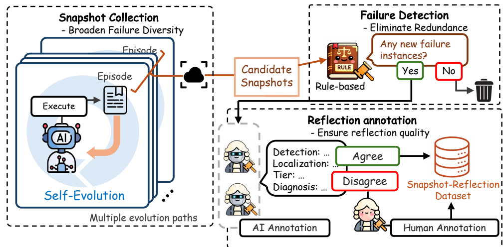
(b) Three-stage dataset construction pipeline
