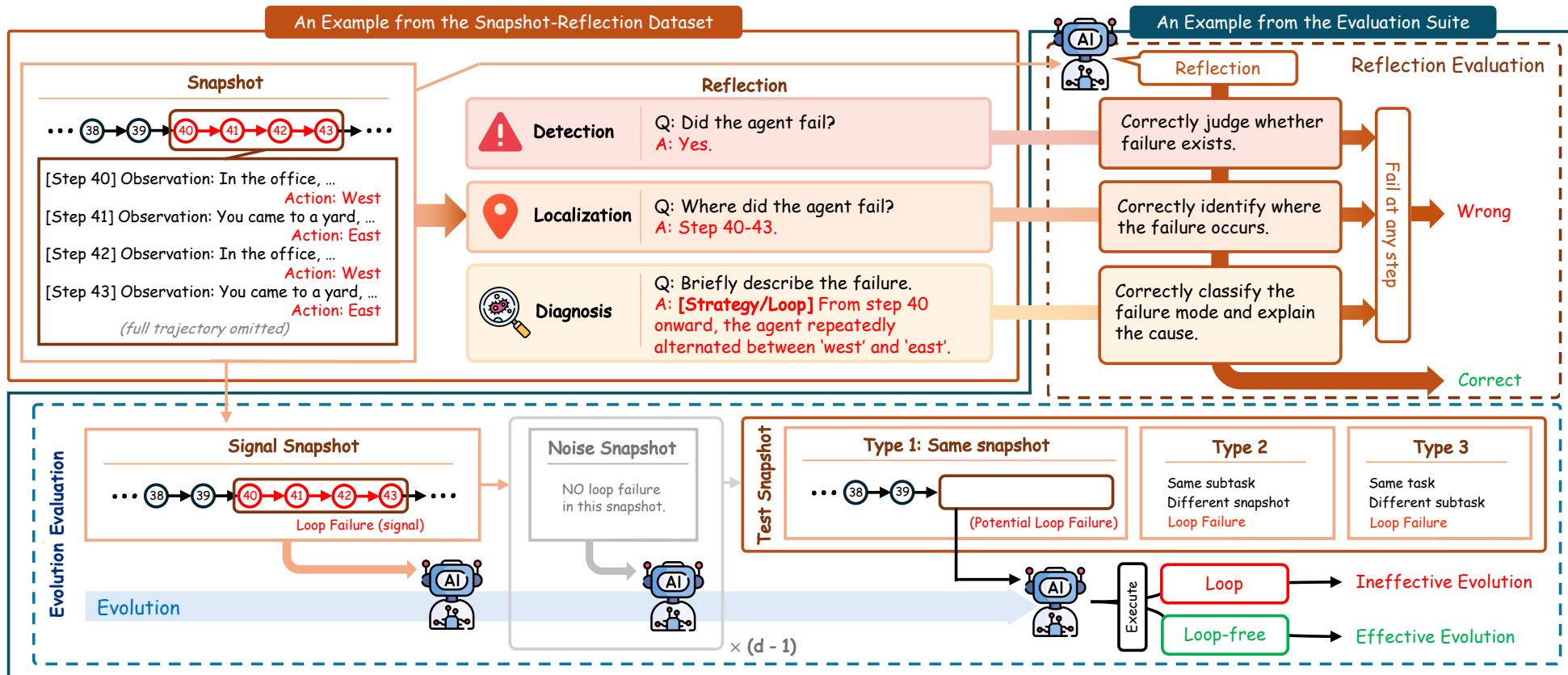
(c) BenchTrace: Snapshot-Reflection Dataset + Evaluation Suite
