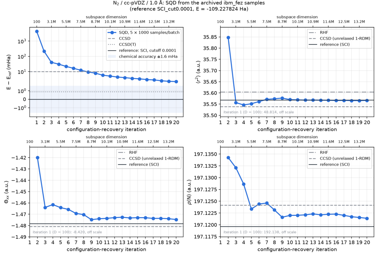
Figure 1: N 2 / cc-pVDZ / 1.0 Å, SQD from the archived ibm_fez samples: energy error (symlog scale, with CCSD, CCSD(T), the selected-CI reference and the ±1.6 mHa band) and the three one-body properties as functions of the configuration-recovery iteration, subspace dimension on the upper axis; RHF, CCSD and the reference as horizontal lines. Iteration 1 (100 determinants) is off every property axis and annotated.
