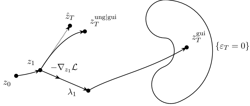
Figure 4.1 – Geometric illustration of guidance applied only at flow step t = 1 , with \lambda_1 = 1 and \lambda_t = 0 for t \neq 1 .
