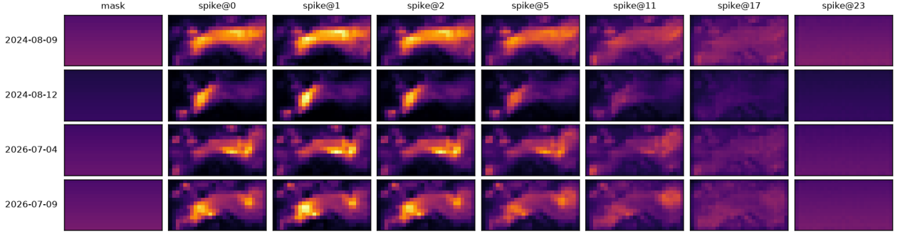
Figure 5.9 – Example normalized spatial distributions used for T1.2. The normalized magnitude of the guidance effect is compared with the prescribed spatial mask for the candidate profiles.
