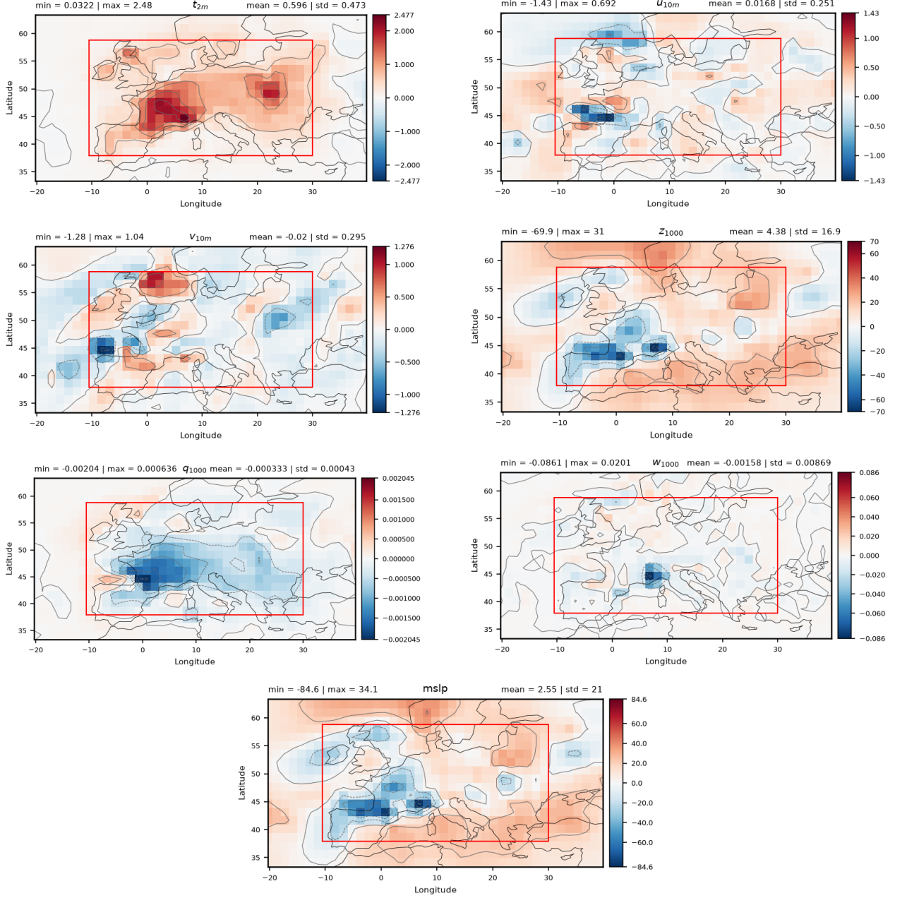
Figure 5.2 – Guidance effect \Delta x^{\text{GE}} for selected atmospheric variables in the representative experiment. Surface variables are shown at \ell = 0 and upper-air variables at 1000 hPa. The maps provide a qualitative view of how an intervention targeted at 2 m temperature propagates to other components of the atmospheric state.
