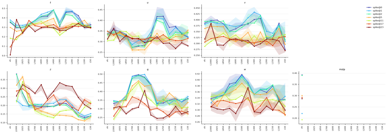
Figure 5.10 – Spatial deviation D_{vl}^\gamma across atmospheric variables and vertical levels for the candidate spike profiles. Solid curves show one ensemble member and bands span the minimum and maximum across the five members.
