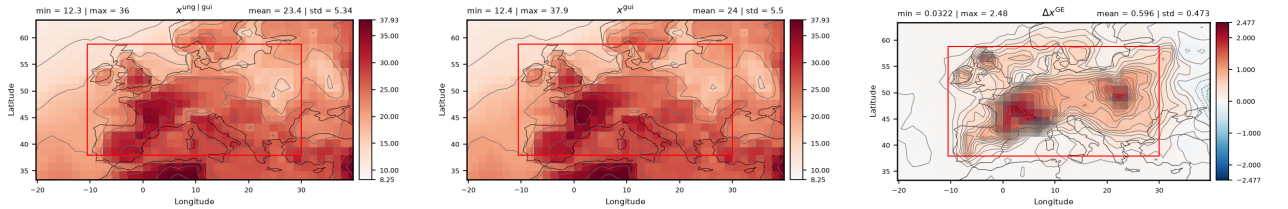
Figure 5.1 – Matched unguided state x^{\text{ung|gui}} (left), guided state x^{\text{gui}} (center), and guidance effect \Delta x^{\text{GE}} (right) for 2m temperature in the representative experiment. The two state panels share a common scale; the guidance effect is shown on a separate diverging scale centered at zero.
