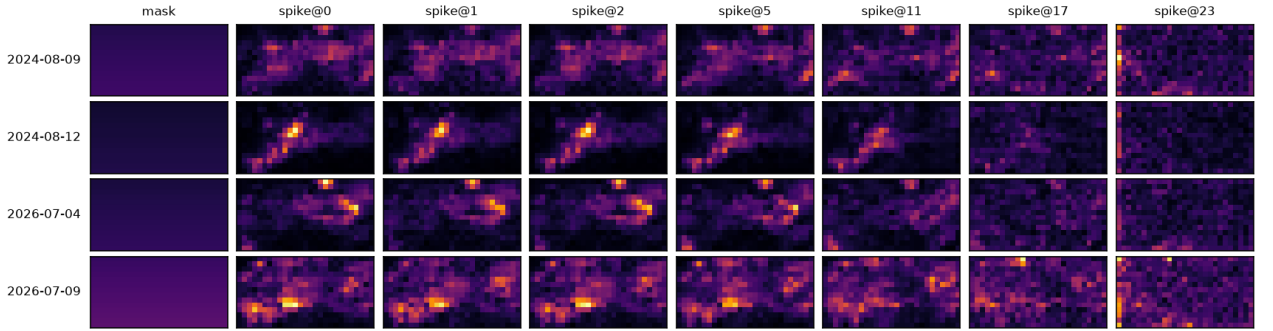
Figure 5.11 – Example spatial distribution of ensemble diversity for the candidate profiles. Each panel shows the pixel-wise standard deviation of the signed guidance effect across ensemble members, normalized for visualization.
