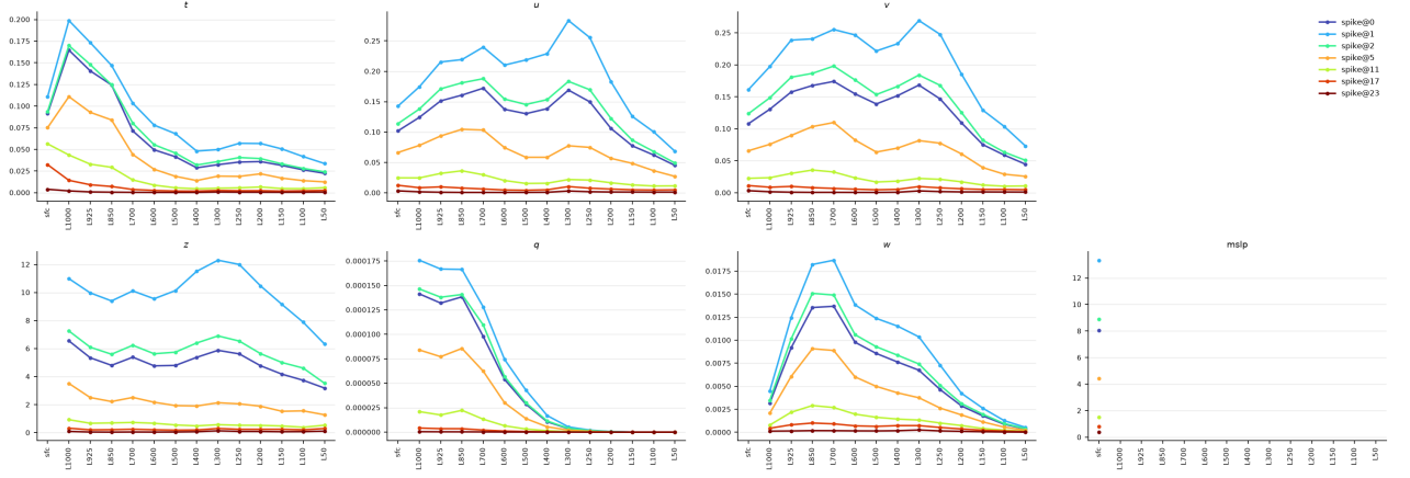
Figure 5.12 – Ensemble diversity across atmospheric variables and vertical levels, measured according to Equation (5.20). No ensemble band is shown because the member dimension is already consumed by the standard deviation.
