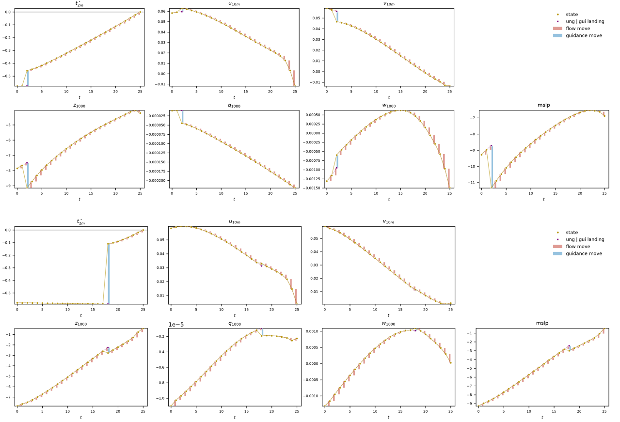
Figure 6.5 – Step-wise decomposition of the guided residual-flow trajectory for spike@1 (top) and spike@17 (bottom), using the same experimental setting and ensemble realization. The panels show the current state, the corresponding unguided-under-guided-context landing, and the contributions of the flow and guidance moves at each flow step.
