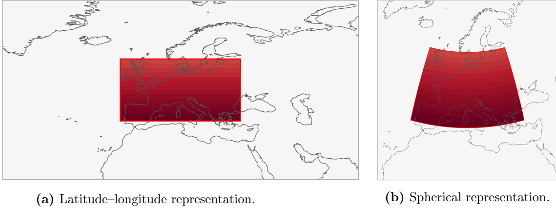
Figure 3.1 – Example of the spatial target mask. The rectangular support determines which grid cells are included, while the latitude-dependent weights account for differences in physical grid-cell area.
