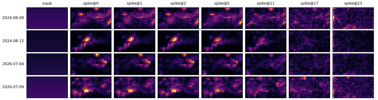
Figure 6.9 – Ensemble variability of the guidance footprint for the candidate spike profiles. Larger values indicate a stronger dependence of the induced perturbation on the stochastic ensemble realization.
