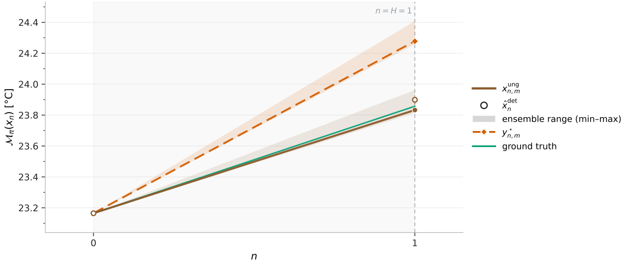
Figure 3.2 – Schematic illustration of the specification procedure. Each unguided reference member defines a baseline trajectory for the targeted regional quantity. Applying the common relative intensity trajectory \rho_{1:H} produces a corresponding member-specific target trajectory over the guided horizon. No target is imposed after weather step H , while the experiment continues until step N .
