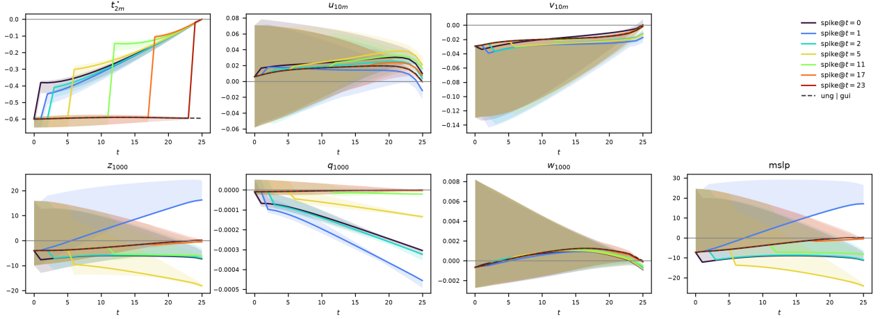
Figure 6.4 – Evolution of the masked guided residual \bar{z}_{t,m,v}^{\text{gui}} for selected atmospheric variables. Curves show the ensemble mean, while the shaded region spans the minimum and maximum across ensemble members. Upper-air variables are shown at their highest available pressure level for visualization.
