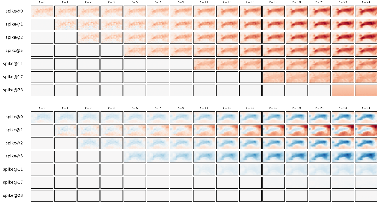
Figure 6.6 – Spatial guidance effect \Delta x^{\text{GE}} for 2m temperature (top) and geopotential at 1000 hPa (bottom) in the representative experiment. The response in geopotential illustrates how an intervention targeted at 2m temperature propagates to another atmospheric variable.
