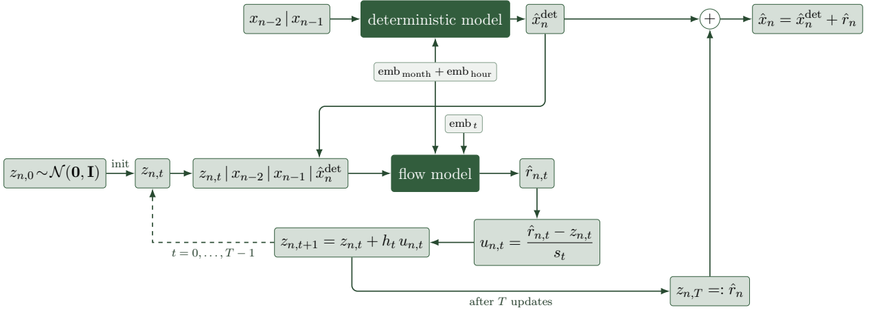
Figure 2.1 – Computational graph of one ArchesWeather forecast step. The deterministic model produces the base forecast \hat{x}_n^{\det} , while the flow model generates the residual through T sampling steps before both components are combined.
