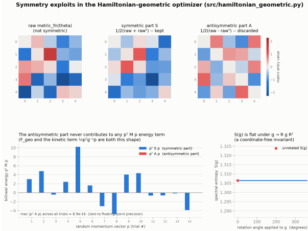
Figure 8: Top: a random raw metric decomposed into symmetric part S (kept) and antisymmetric part A (discarded). Bottom-left: p^\top S p varies with p ; p^\top A p is zero to floating-point precision for every p . Bottom-right: spectral entropy S(g) is flat under rotation of g .
