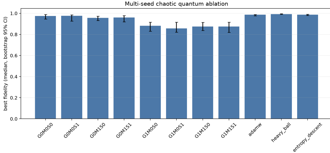
Figure 8: Median fidelity with bootstrap 95% confidence intervals, paired 10-seed replication, same task as Table 11.
