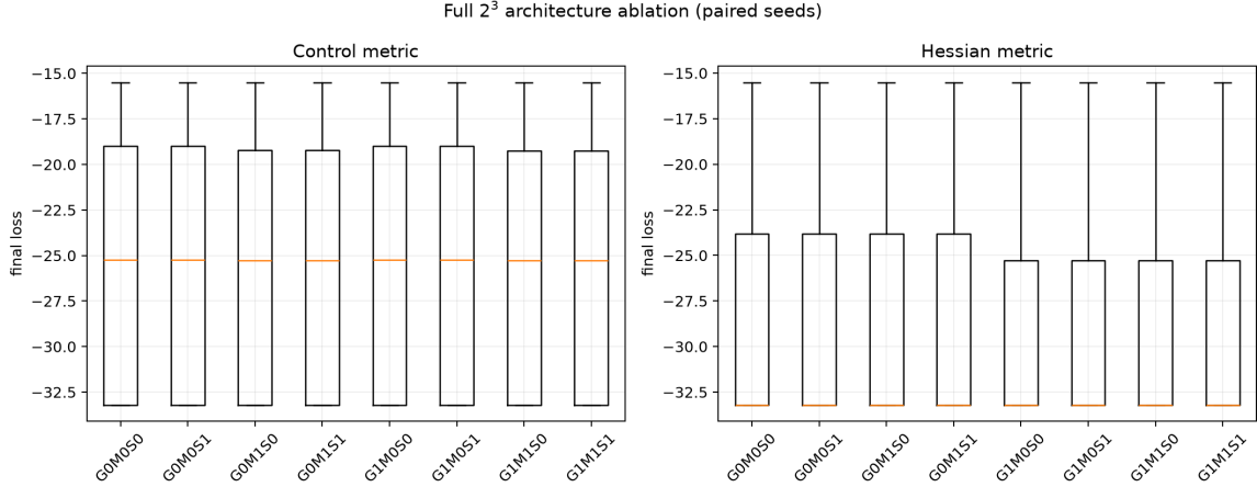
Figure 7: Independent replication: final-loss distributions across the full 2^3 factorial, control vs. Hessian metric. Compare with the plotting-artifact note in §11.
