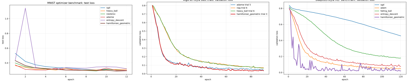
Figure 1: Classical benchmark loss curves. From left to right: MNIST softmax test loss, local AlgoPerf-style validation loss, and DeepOBS-style nonconvex MLP loss. These plots complement Tables 3–5 by showing whether each final number came from smooth convergence, late-training instability, or a short-budget plateau.
