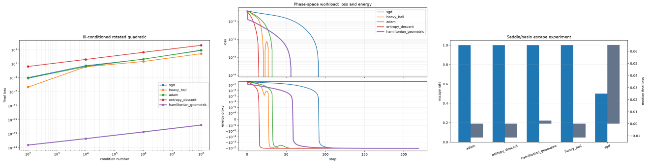
Figure 4: Mechanism-focused diagnostic graphs. Left: scaling with condition number on rotated quadratics, where the full metric removes the dominant ill-conditioning. Middle: double-well loss and Hamiltonian-style energy traces. Right: saddle/basin escape behavior across random starts. These plots separate “works because the geometry is exploitable” from “wins because of a tuned learning rate on one task.”
