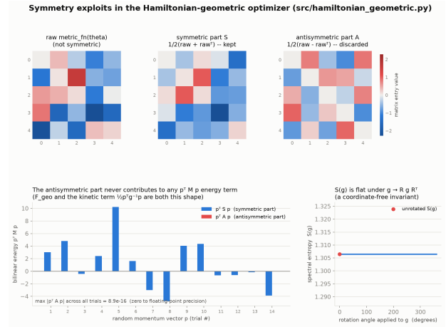
Figure 6: Top: a random raw metric decomposed into symmetric part S (kept) and antisymmetric part A (discarded). Bottom-left: p^T S p varies with p ; p^T A p is zero to floating-point precision for every p . Bottom-right: spectral entropy S(g) is flat under rotation of g .
