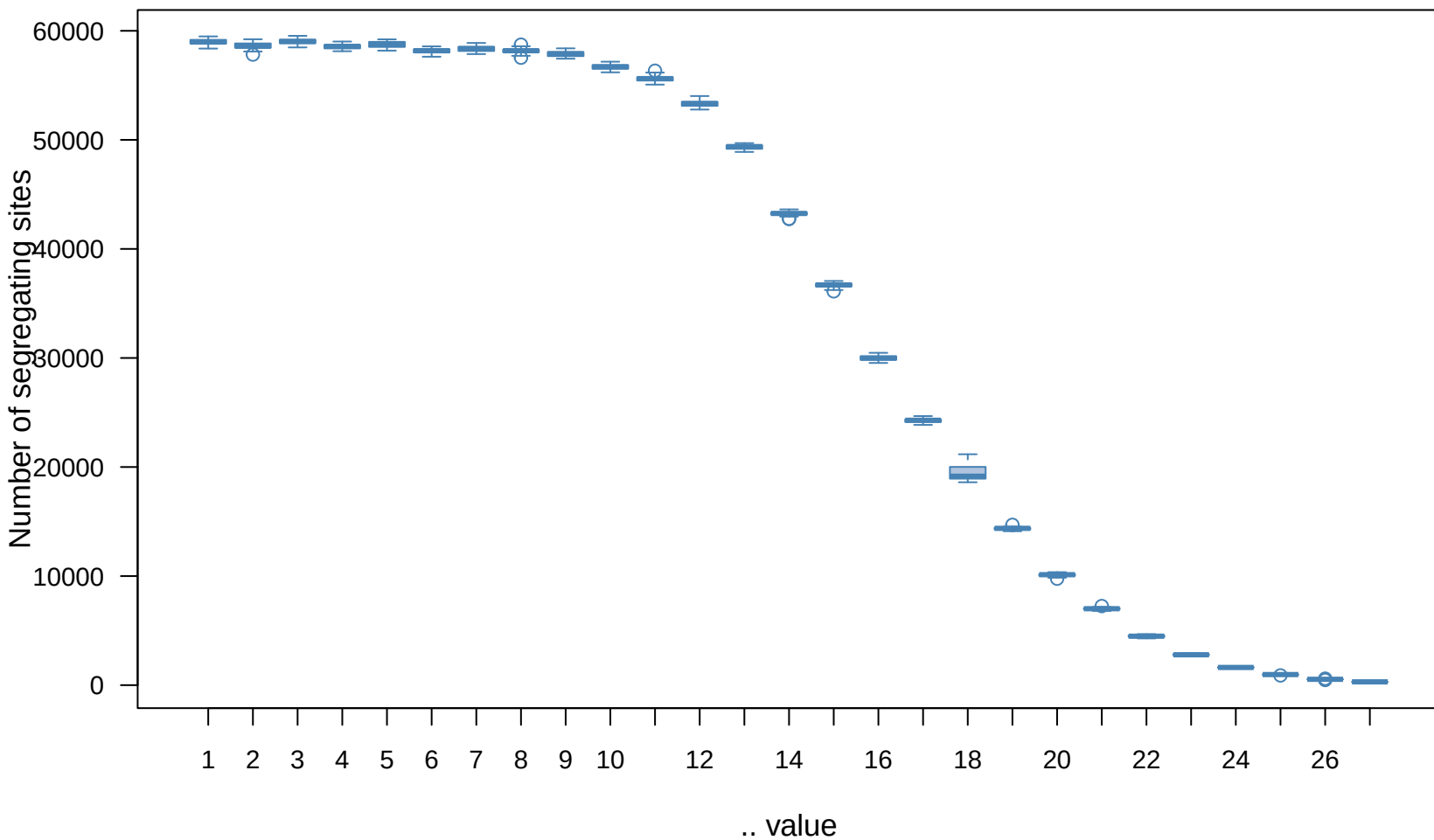
Distribution across 50 repetitions per .. value
