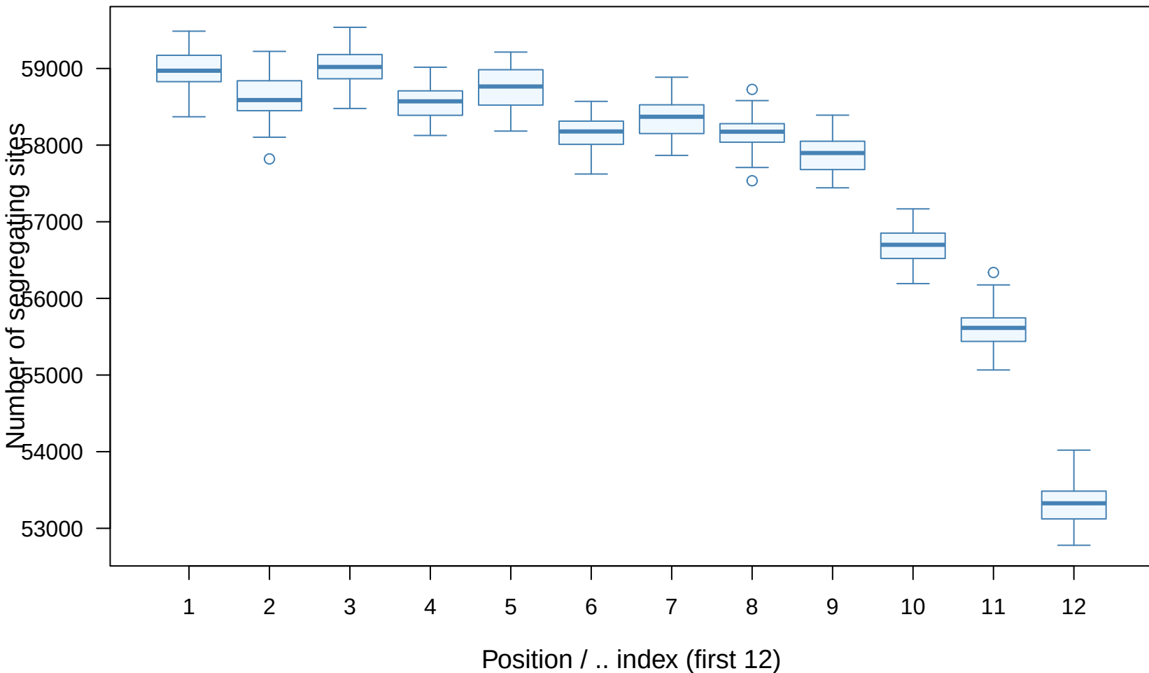
Distribution across 50 repetitions (positions 1...12)
