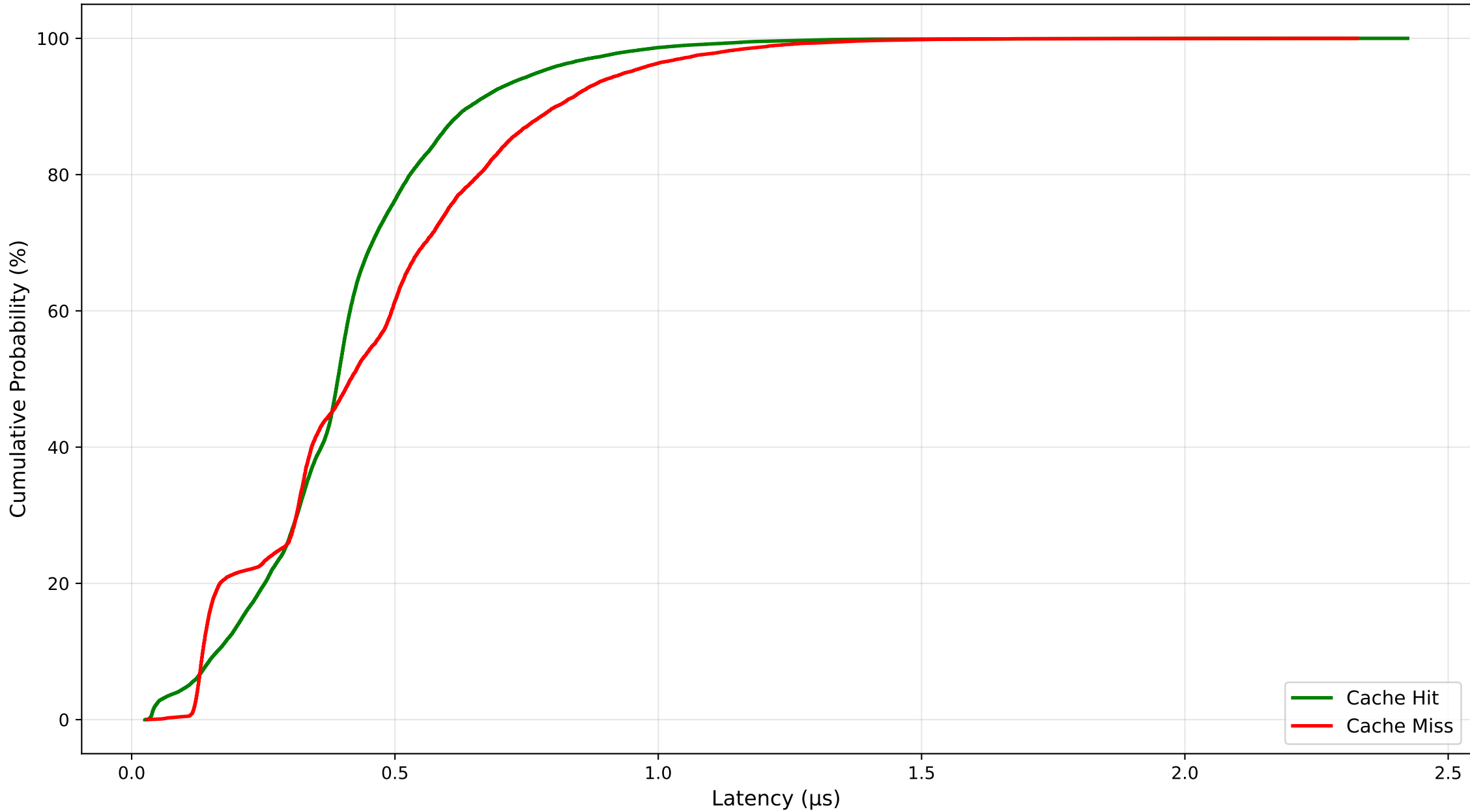
assoc_find() Latency CDF - Hits vs Misses
