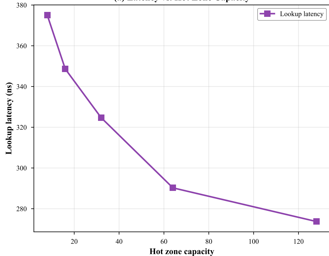
(a) Latency vs. Hot Zone Capacity
