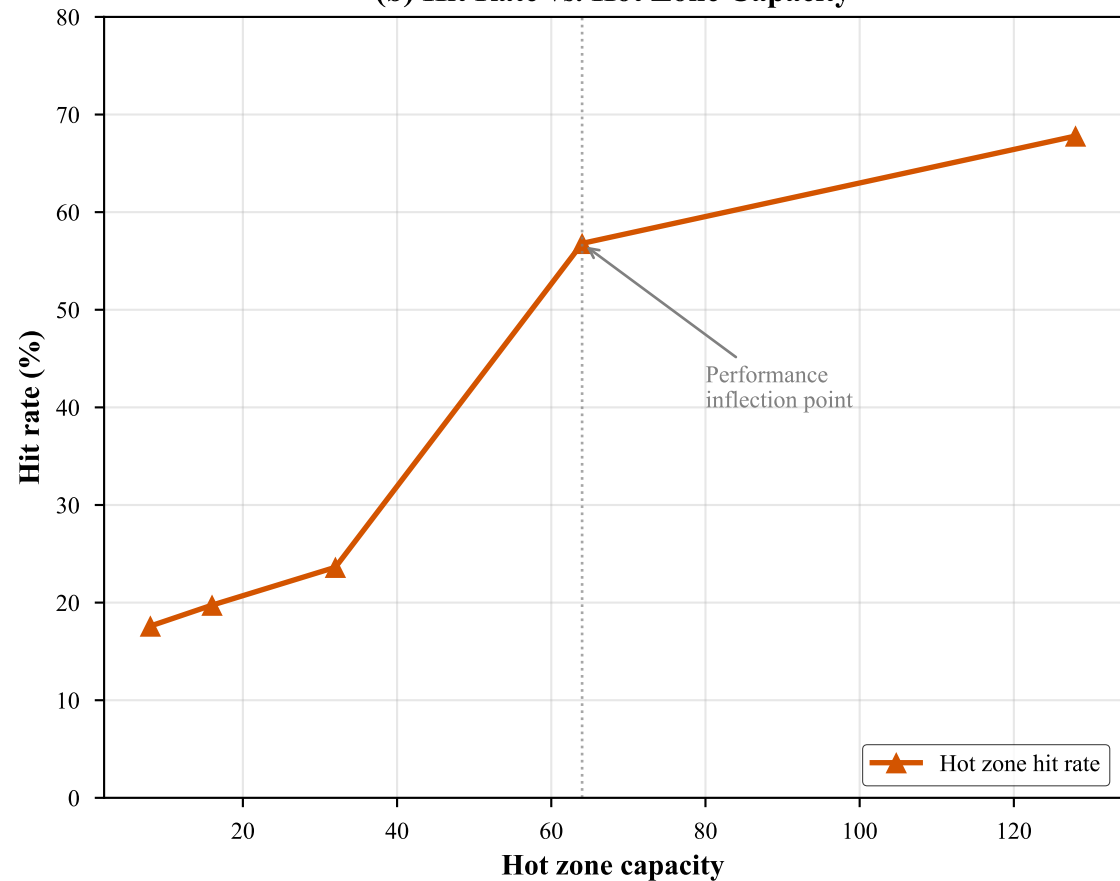
(b) Hit Rate vs. Hot Zone Capacity
