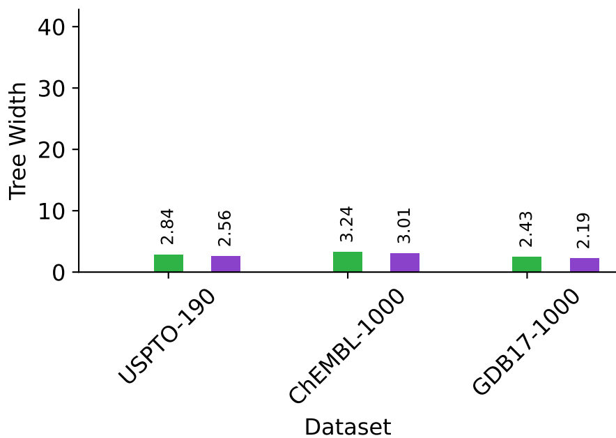
Solved Average Clustered Tree Width
