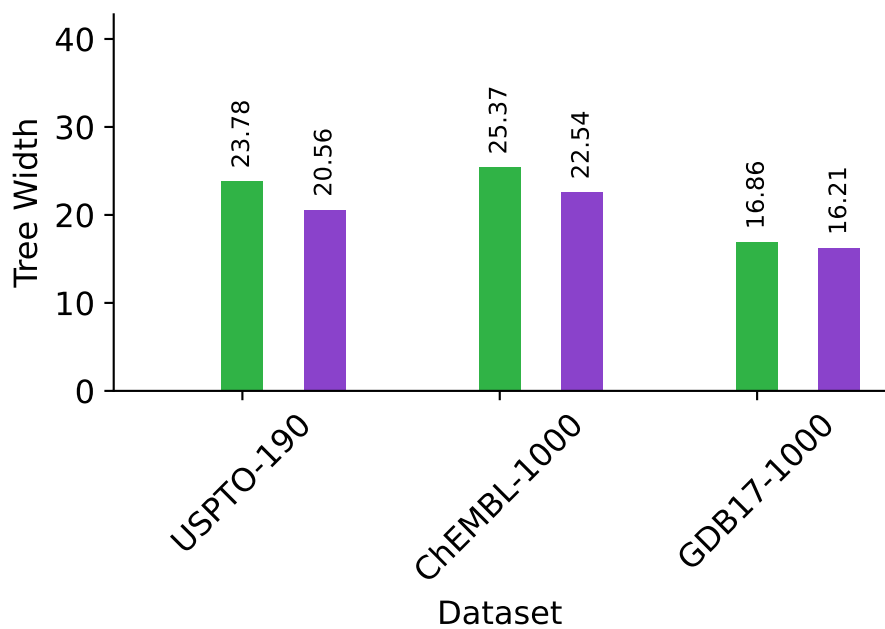
Solved Average Normal Tree Width
