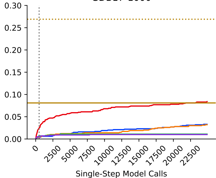
GDB17-1000
