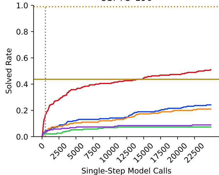
USPTO-190
