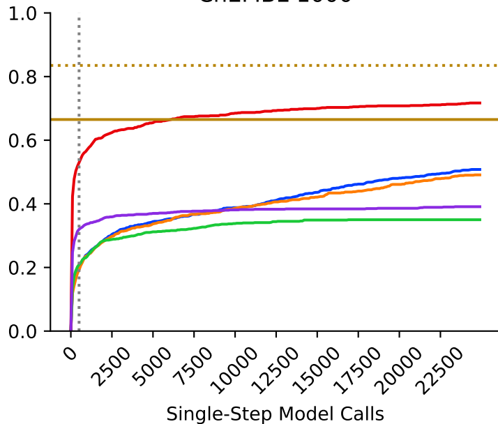
ChEMBL-1000
