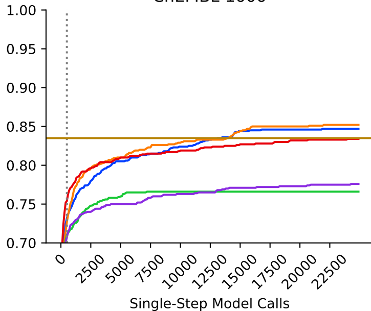
ChEMBL-1000
