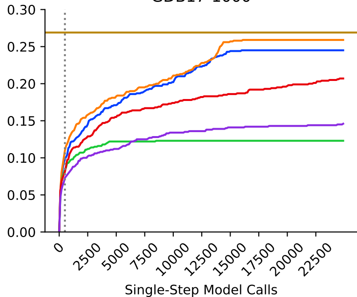
GDB17-1000
