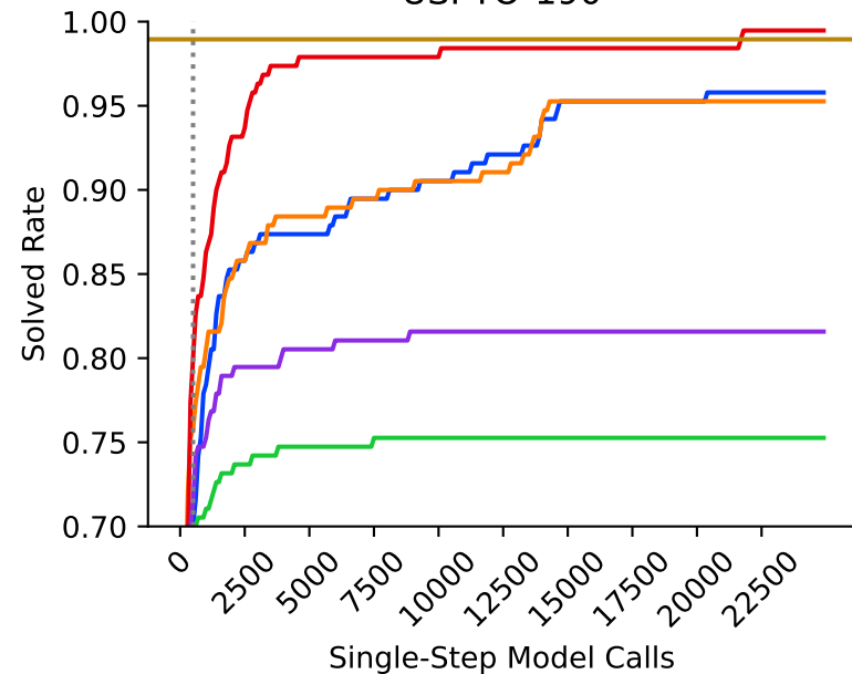
USPTO-190
