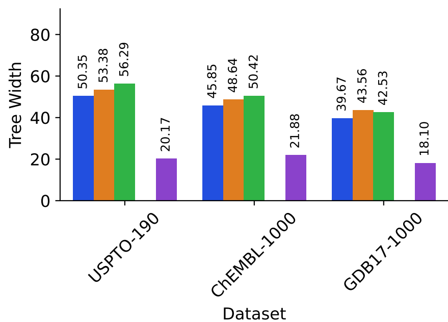
Solved Average Normal Tree Width
