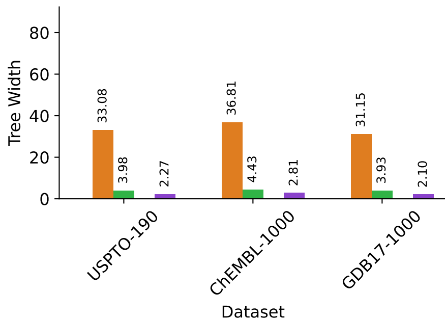
Solved Average Clustered Tree Width
