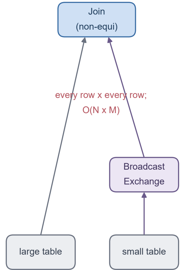
BroadcastNestedLoopJoin
