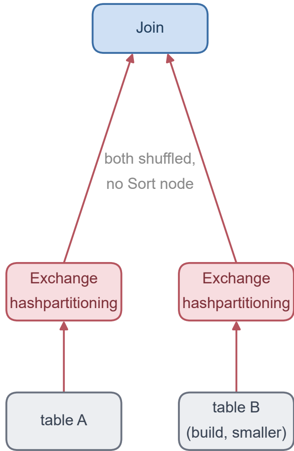
ShuffledHashJoin
