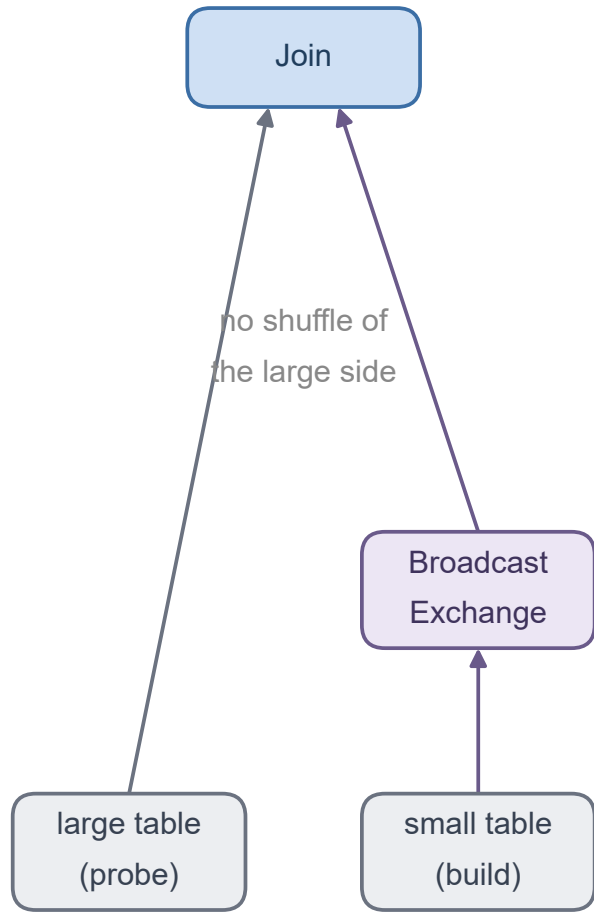
BroadcastHashJoin
