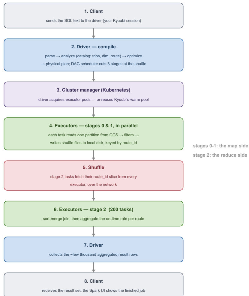
Figure 1.2: The specimen query from submission to result. The driver compiles and schedules but never touches the data; executors do all the reading, shuffling, and computing; the cluster manager only supplies the pods.
