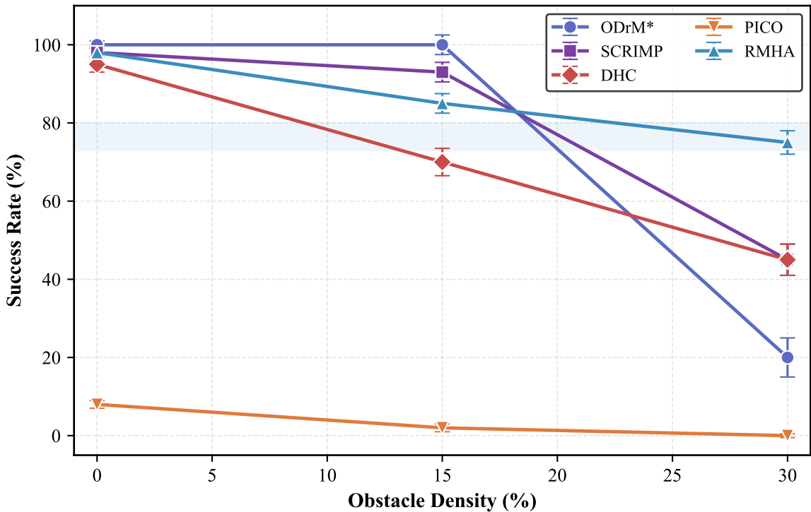
Success Rate Comparison Across All Methods (128 Agents, 40×40 World)
