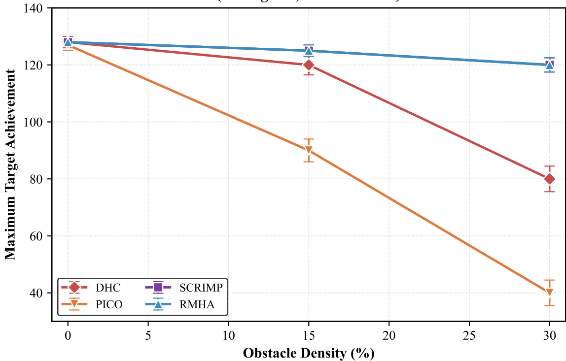
Maximum Target Achievement Across Methods (128 Agents, 40×40 World)
