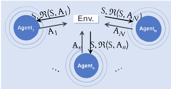
(b) MG
