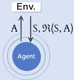
(a) MDP
