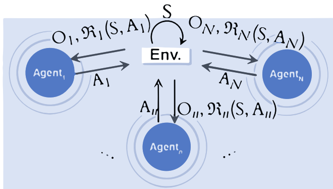
(c) POMG
