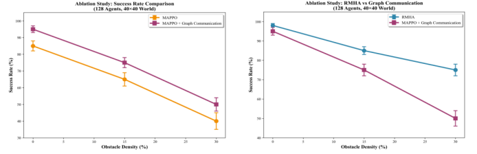
(a) MAPPO vs. Graph Comm
