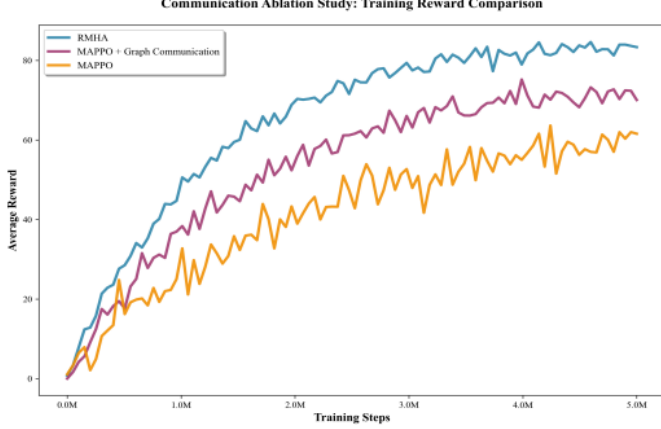
Fig. 7. Communication ablation: training reward curves.
