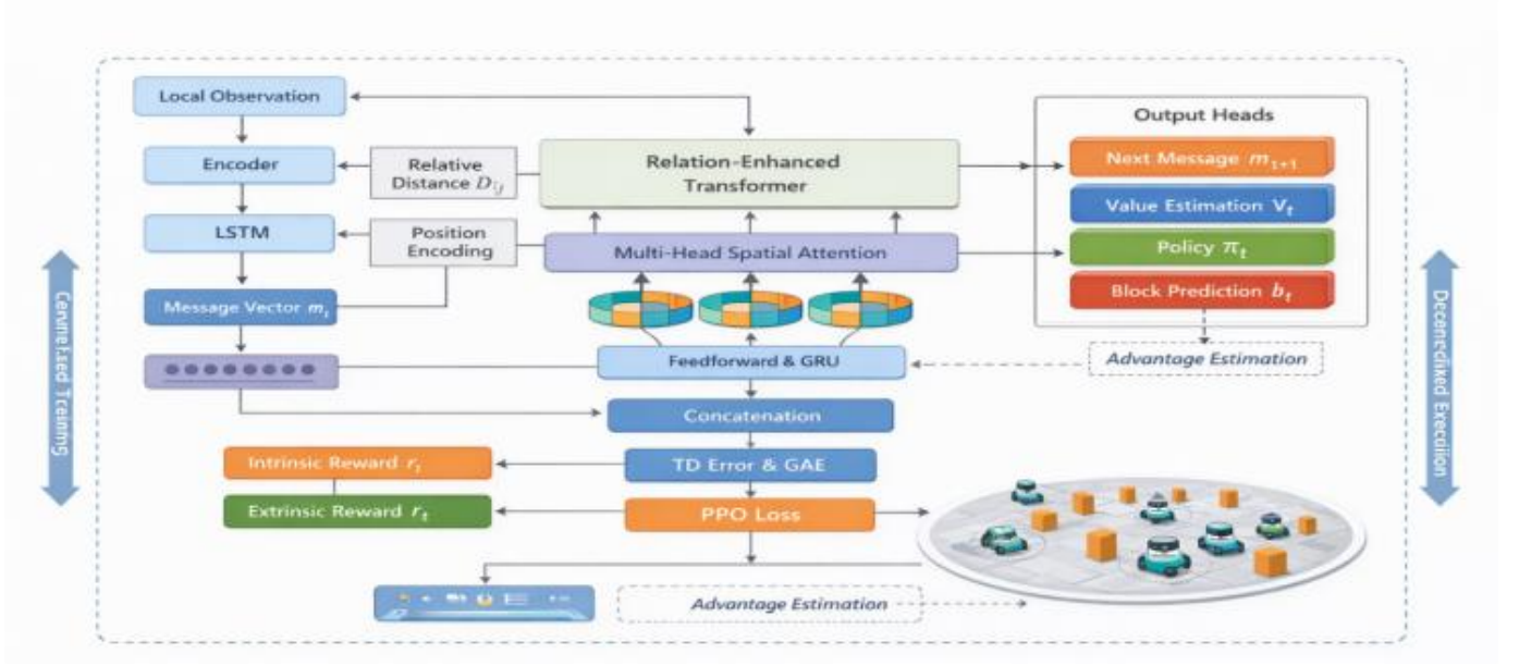
Fig. 4. Network architecture of rmha integrated with MAPPO.
