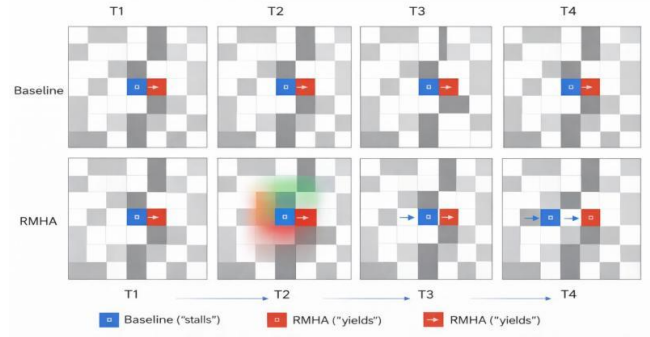
Fig. 12. Deadlock resolution in a narrow corridor. At T_1 , robots A and B enter a conflict; the baseline leads to deadlock by T_2 – T_3 . Under rmha, robot A yields at T_3 , allowing B to pass, and both proceed by T_4 .
