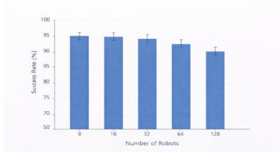
Fig. 6. Success rate of rmha under different robot counts.
