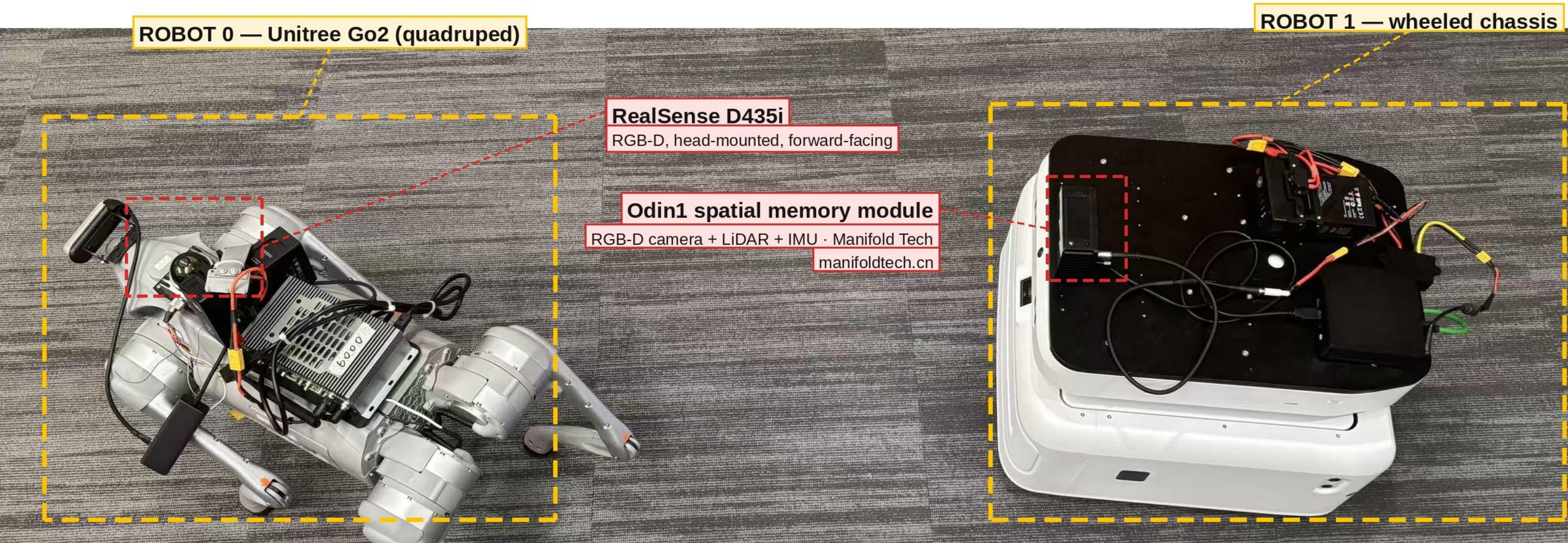
Fig. Real-world experiment platforms. Robot 0 is a Unitree Go2 quadruped carrying a head-mounted Intel RealSense D435i RGB-D camera and onboard compute. Robot 1 is a wheeled delivery chassis carrying an Odin1 spatial memory module (RGB-D camera + LiDAR + IMU, Manifold Tech, manifoldtech.cn ) and onboard compute on its rear deck. Both platforms run local planning/control onboard; a central hub only publishes expiring targets.
