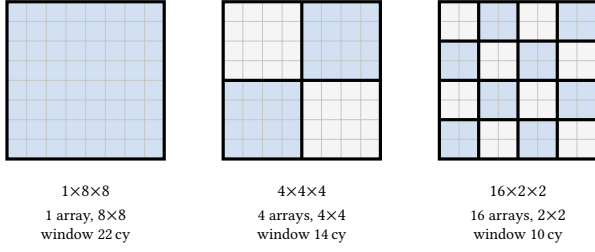
Figure 2: Output-matrix partitioning under a fixed 64-PE budget. The 8x8 output is split into M^2 non-overlapping blocks (shaded), each computed by a dedicated n \times n sub-array with n = 8/M . All three configurations use the same 64 PEs; smaller blocks shorten the wavefront path to the corner PE, cutting the per-tile compute window from 22 cycles ( 1 \times 8 \times 8 ) to 10 cycles ( 16 \times 2 \times 2 ).
