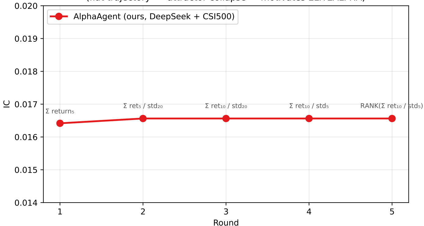
Figure 5: Per-round IC of AlphaAgent's mining loop on CSI 500 (flat trajectory \Rightarrow attractor collapse — motivates ELITEALPHA)
