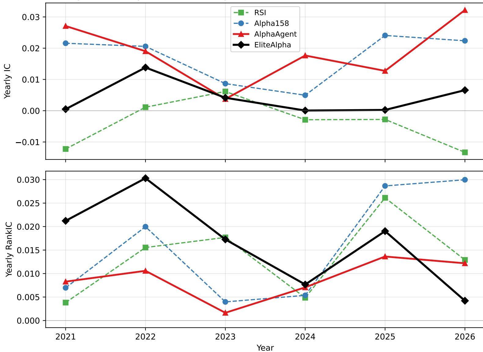
Figure 4: Yearly IC and RankIC by Factor Source on CSI 500 (2021-06 ~ 2026-05)
