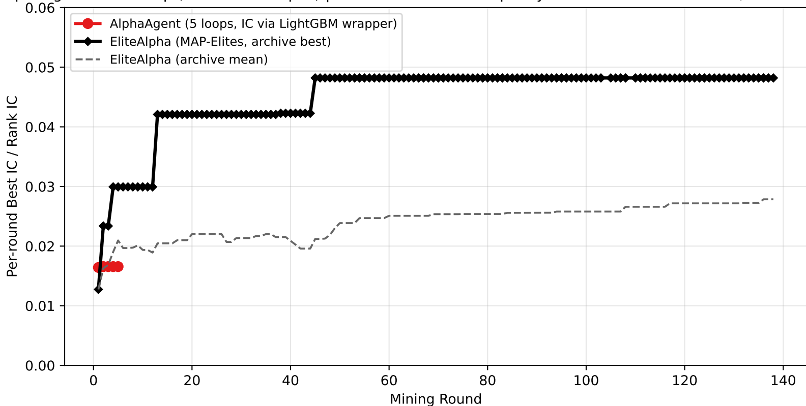
Figure 5: Mining trajectory comparison on CSI 500
