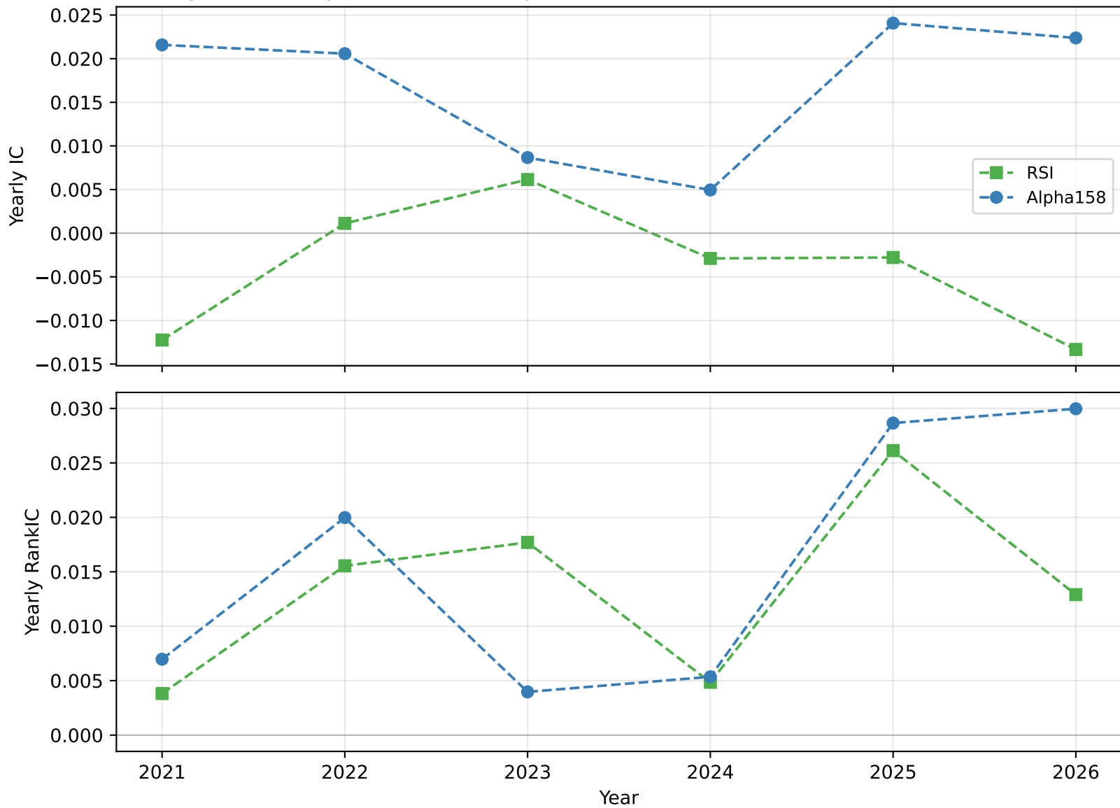
Figure 4: Yearly IC and RankIC by Factor Source on CSI 500 (2021-06 ~ 2026-05)
